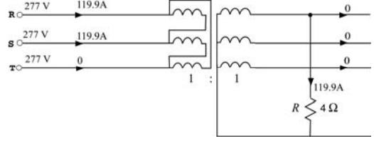
Fig. 2. Example of circuit with resistive load
