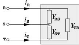
Fig. 5. Equivalent circuit of three-phase, static linear load
