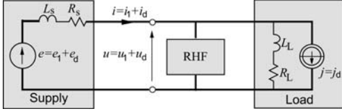
Fig. 2. One phase equivalent circuit of the system in Fig. 1.
