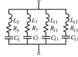
Fig. 3. Four branch RHF structure
