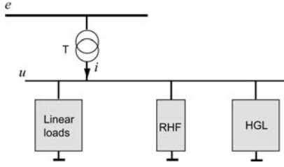
Fig. 1. Distribution system bus with harmonic generating load and resonant harmonic filter
