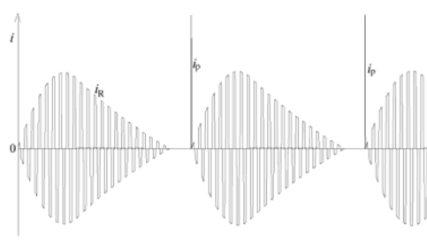
Figure 2. Example of pulsed load supply and output currents
