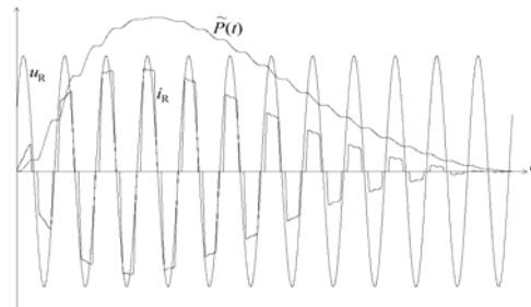
Figure 4. Variation of the running active power
