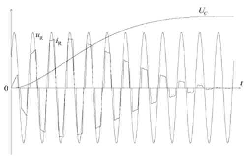
Figure 3. Supply voltage and current of a pulsed load and the capacitor voltage
