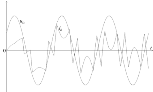
Figure 6. Distorted current waveform
