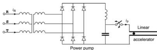
Figure 1. Example of a pulsed load
