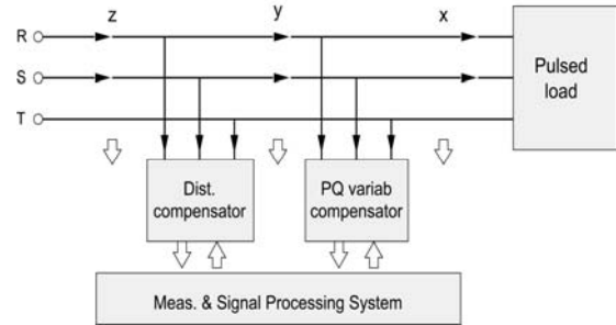
Figure 7. Structure of a hybrid compensator of pulsed loads
