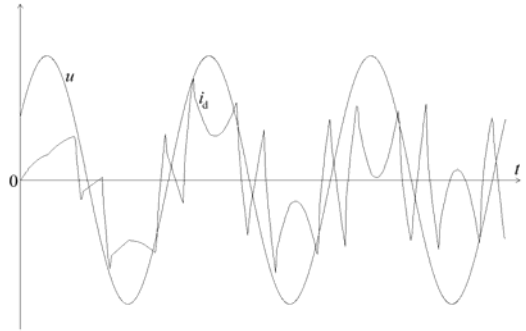
Figure 8. Predicted distorted current waveform
