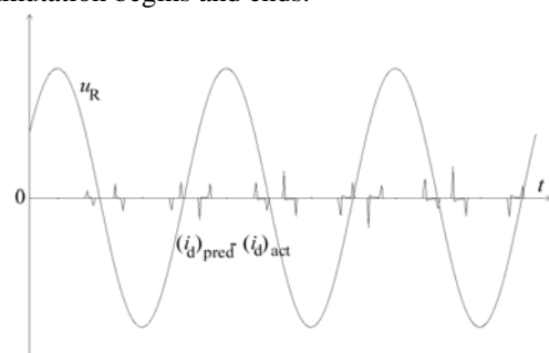
Figure 9. Difference between predicted and actual distorted current at sampling rate of 128 samples per period T
